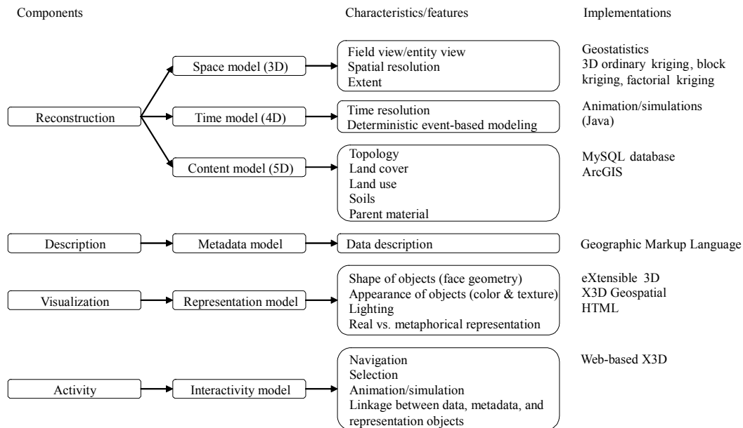
Fig.2 A system design describing the components, models, and characteristics of our approach and how they are implemented
